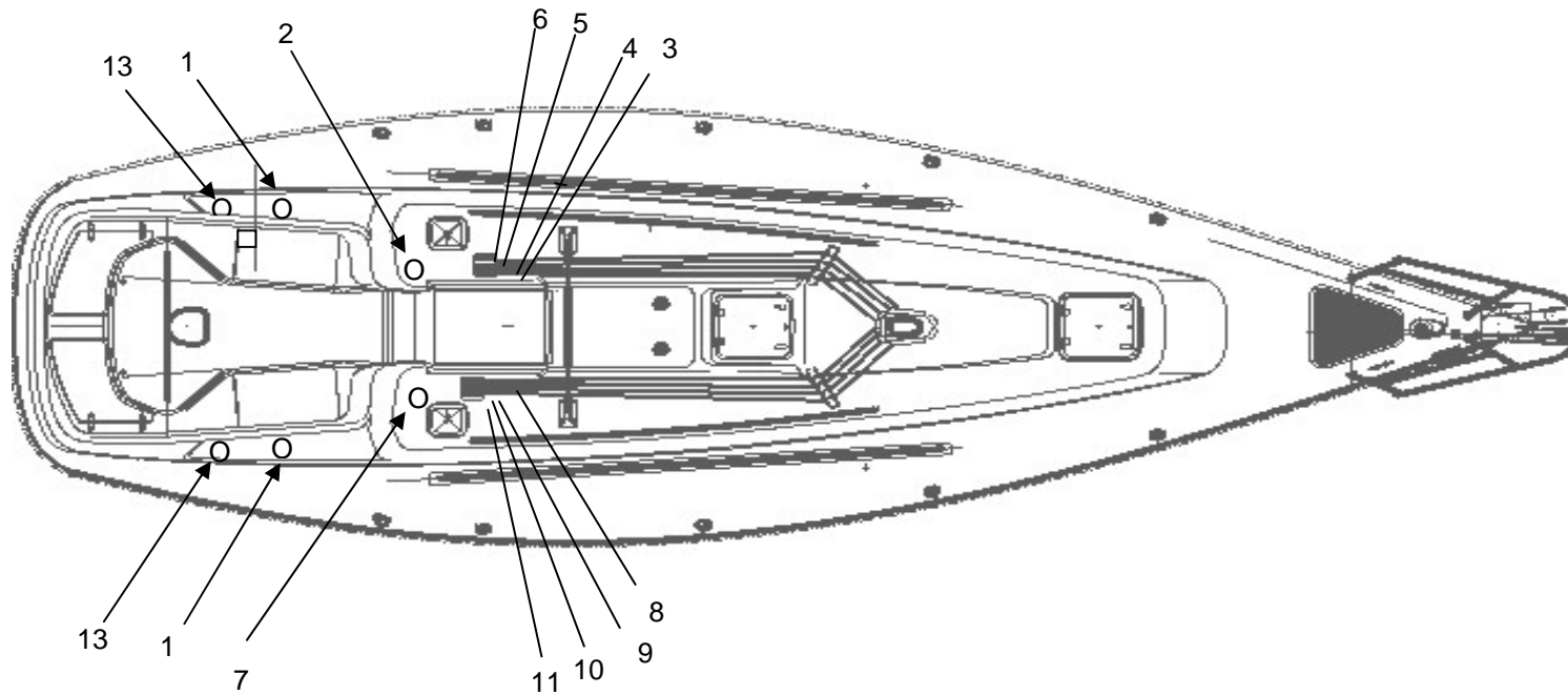
S386 SPINNGEAR DECK LAYOUT
