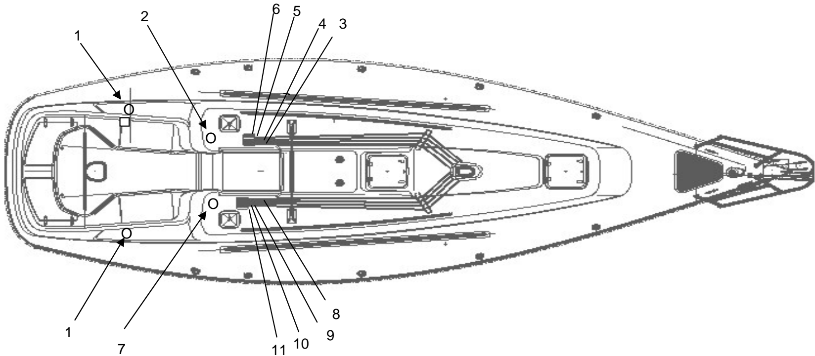
S386 STANDARD DECK LAYOUT
